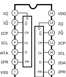
IC402 : TC4013BP Dual D Flip Flop
