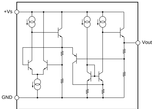
IC301 : LM61CIZ Temperature Sensor
