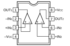
IC901: μPC4570G2 Dual OP-Amp
