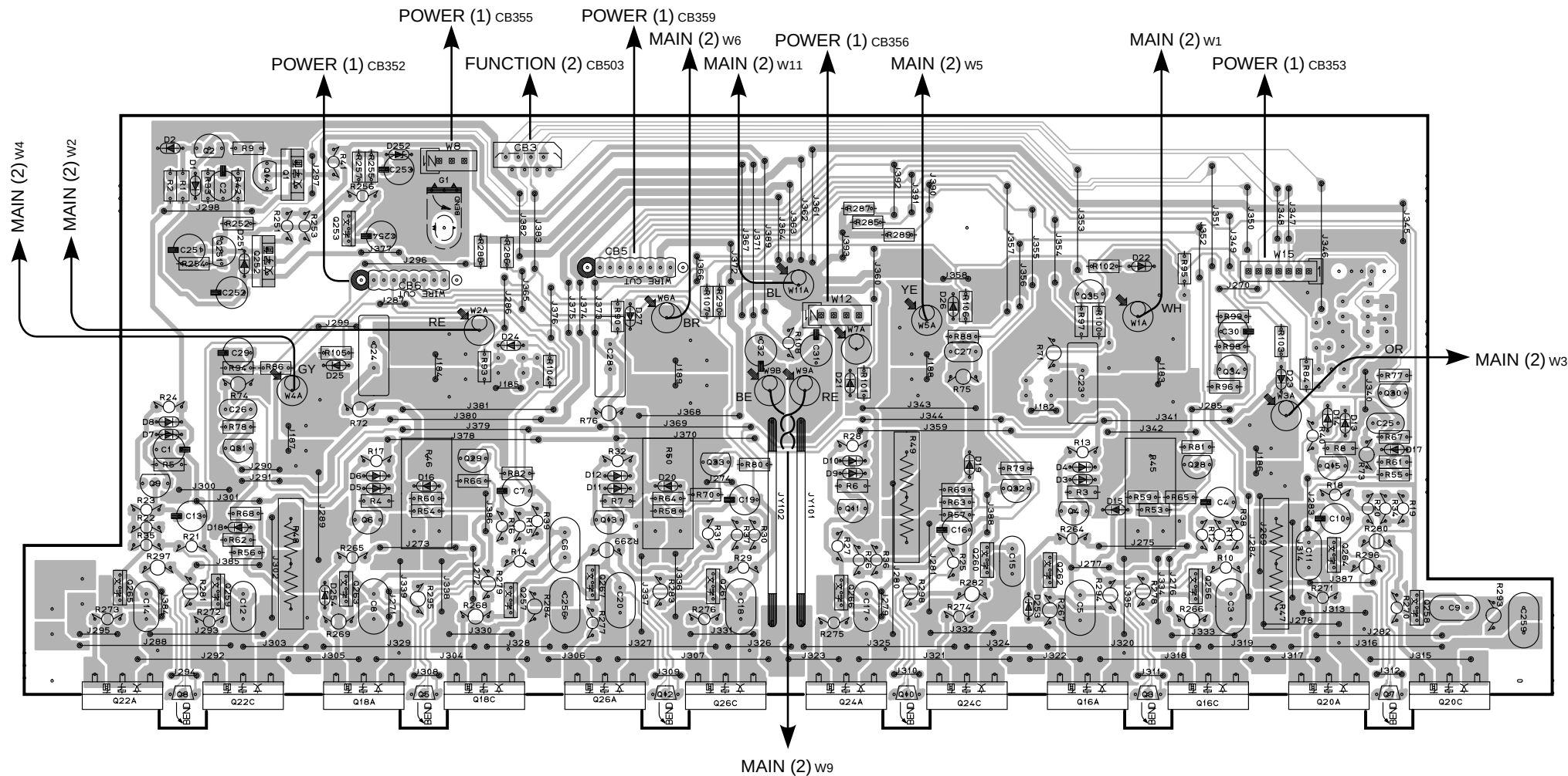
MAIN (1) P.C.B. (Lead Type Device)
